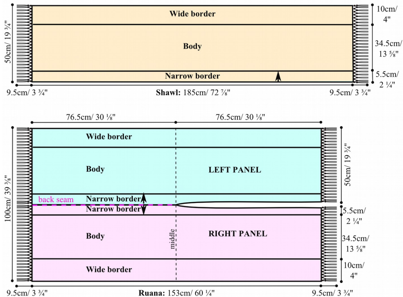
Schematic 1. Ruana and shawl measurements.
